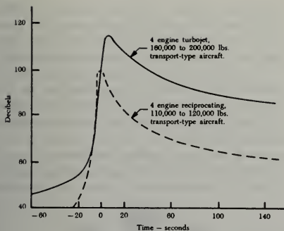
FIGURE 2-39. Noise levels.
